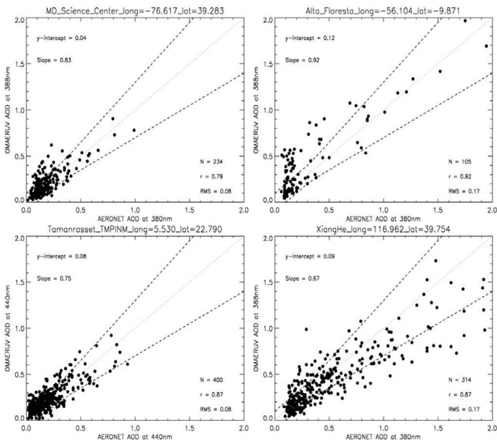
Figure 11: OMAERUV-AERONET comparison of aerosol optical depth. For the comparison at Tamanrasset, the OMI retrieval has been converted to 440 nm.
