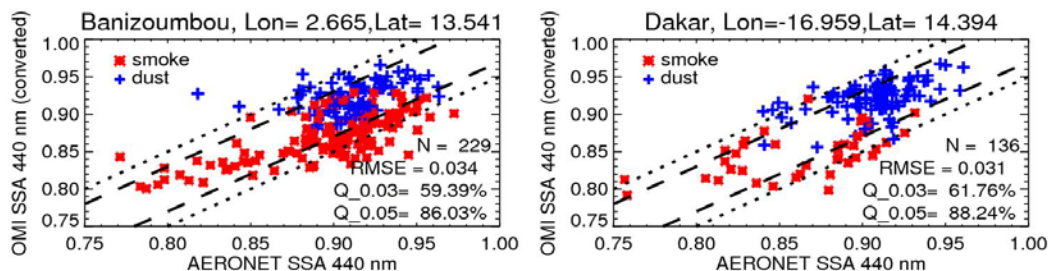
Figure 12: OMAERUV-AERONET comparison of single scattering albedo
