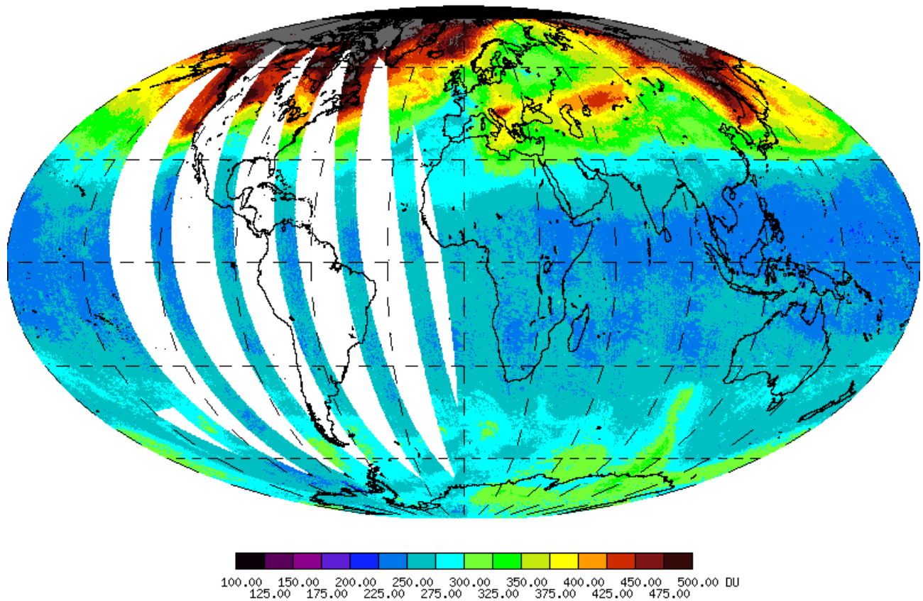
OMDOA03 Total Column Ozone on 2007-02-27 for Orbits 13932-13946
