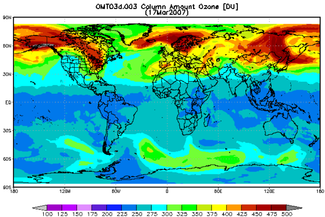
Figure 14: An Image of Column Ozone Generated Using OMI-Giovanni
