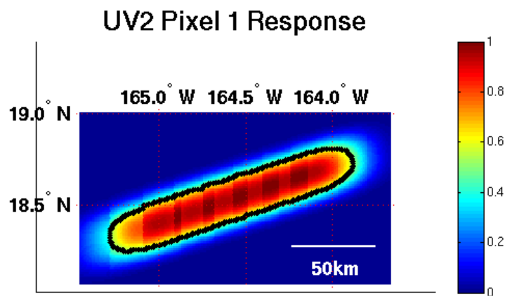
Figure 9: Approximation of Pixel Shape
